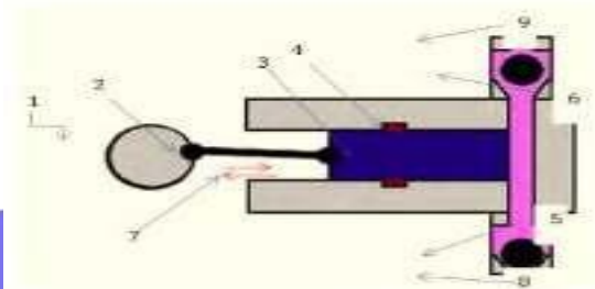
Gambar 40. Cara kerja pompa plunyer (sumber gambar. http://iwanaiik.wordpress.com/2010/11/29/pompa-3/ )
