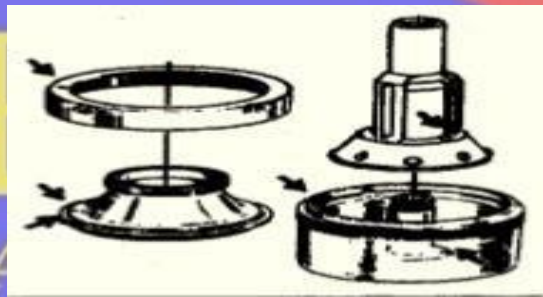
Gambar 4. Bowl, distributor, disc (sumber gambar. http://kapal-cargo.blogspot.com/2011/03/oil-purifier-kapal.html )
