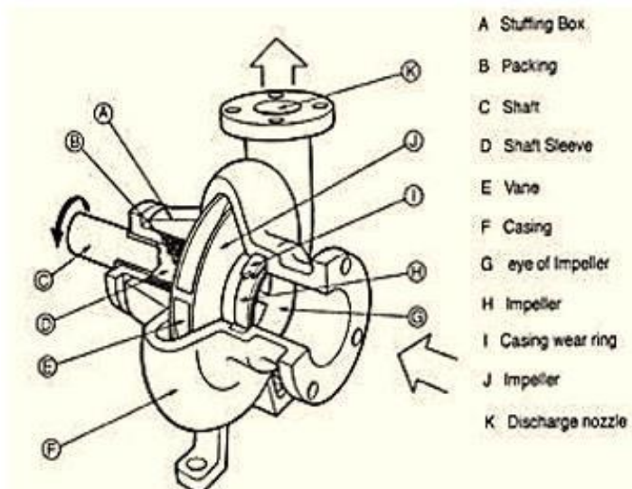
Gambar 44. Gambar bagian-bagian utama pompa sentrifugal (sumber gambar. http://tekimku.blogspot.com/ )
