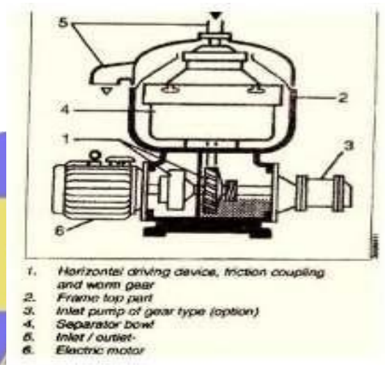
Gambar 3. Skematik sentrifuse jenis disc bowl (sumber gambar. http://kapal-cargo.blogspot.com/2011/03/oil-purifier-kapal.html )
