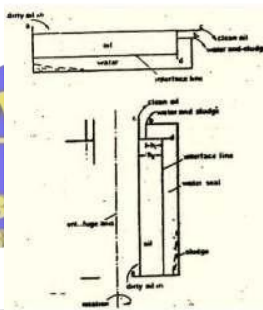
Gambar 1. Prinsip dasar kerja purifier (sumber gambar. http://kapal-cargo.blogspot.com/2011/03/oil-purifierkapal.html )
