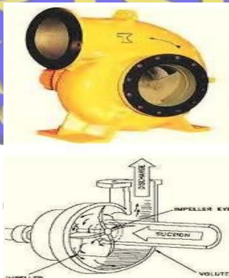
Gambar 41. Volute centrifugal pump (sumber gambar. https://www.google.com/#q=volute+centrifugal+pump+design )
