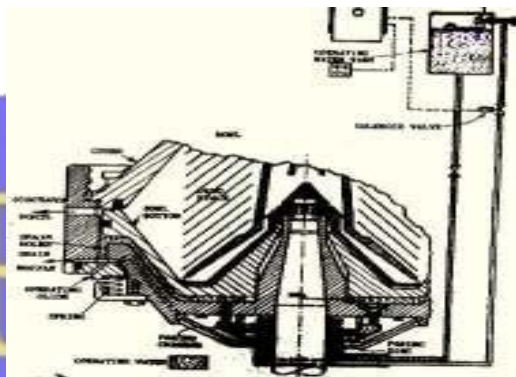
Gambar 11. Cara kerja purifier jenis self cleaning (sumber gambar. http://kapal-cargo.blogspot.com/2011/03/oil-purifier-kapal.html )
