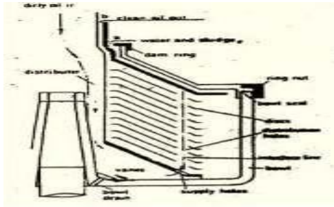
Gambar 7. Purifier (sumber gambar. http://kapal-cargo.blogspot.com/2011/03/oil-purifier-kapal.html )
