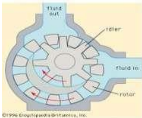
Gambar 46. Pompa roda gigi internal (sumber gambar. http://agungfauzi.blogspot.com/2010/03/gear-pump-pomparoda-gigi.html )
