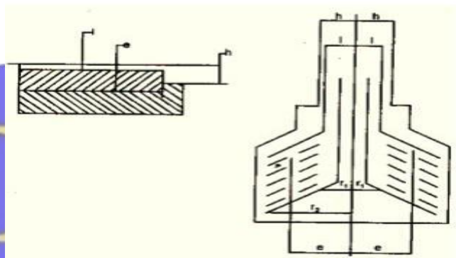
Gambar 2. Pembersihan di tangki endap sentrifuse (sumber gambar. http://kapal-cargo.blogspot.com/2011/03/oil-purifierkapal.html )
