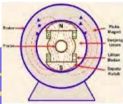
Gambar 35. Badan ( body ) generator arus searah.
