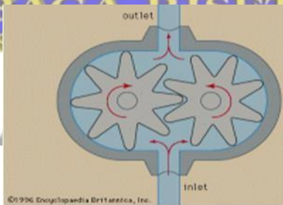
Gambar 45. Pompa roda gigi eksternal (sumber gambar. http://agungfauzih.blogspot.com/2010/03/gear-pumppompa-roda-gigi.html )
